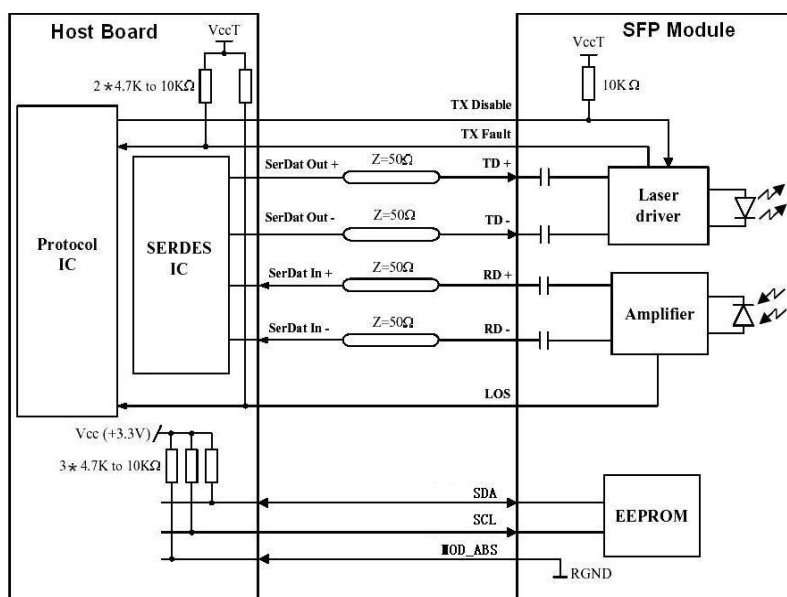
Recommended Host Board Power Supply Circuit
