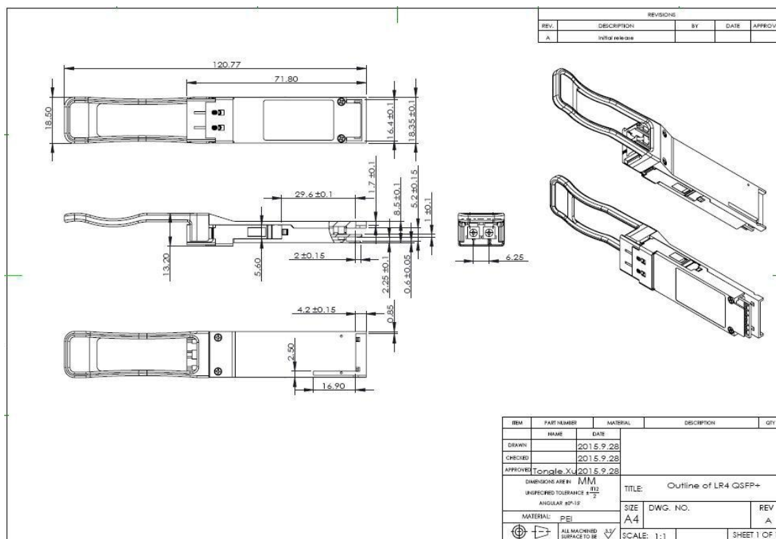
Mechanical Drawing
