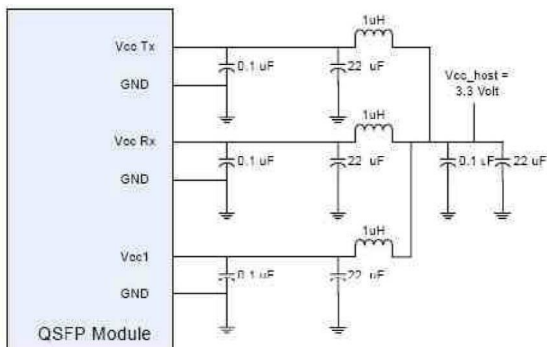
SFP Host Recommended Circuit
