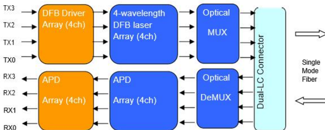
40Gb/s QSFP ZR4-Lite Transceiver Block Diagram
