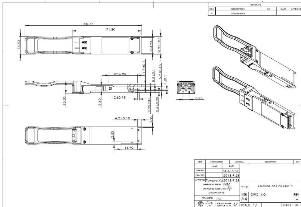
Mechanical Drawing
