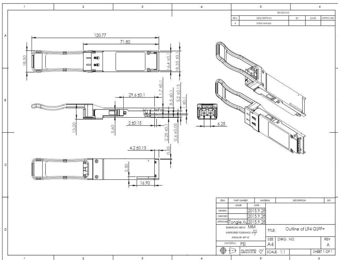
Mechanical Drawing
