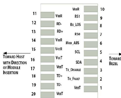
Figure2:Diagram of Host Board Connector Block Pin Numbers and Names
