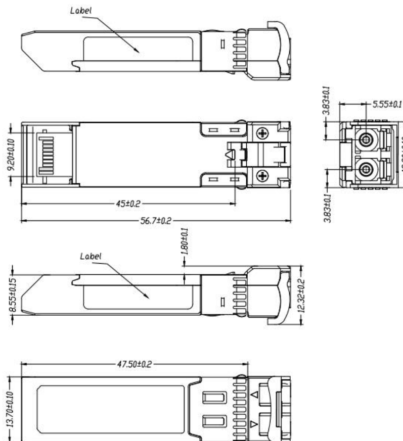
Mechanical Drawing
