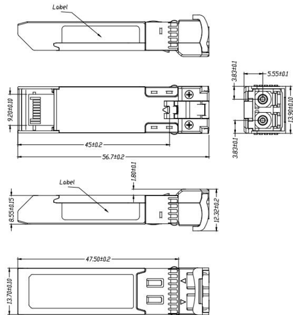
Mechanical Drawing
