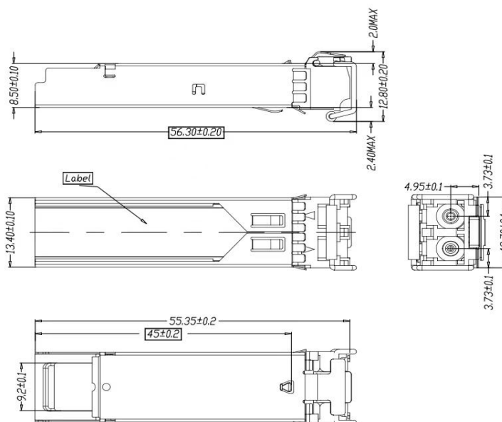
Mechanical Drawing
