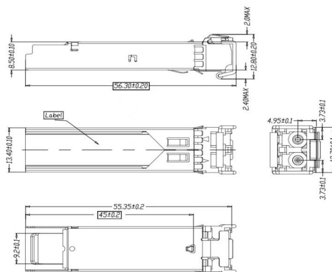
Mechanical Drawing
