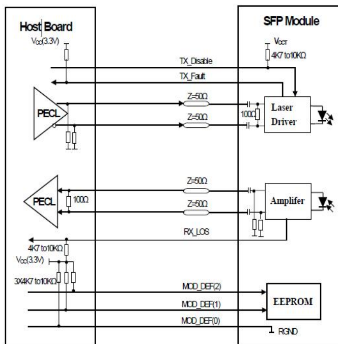
Recommended Host Board Power Supply Circuit
