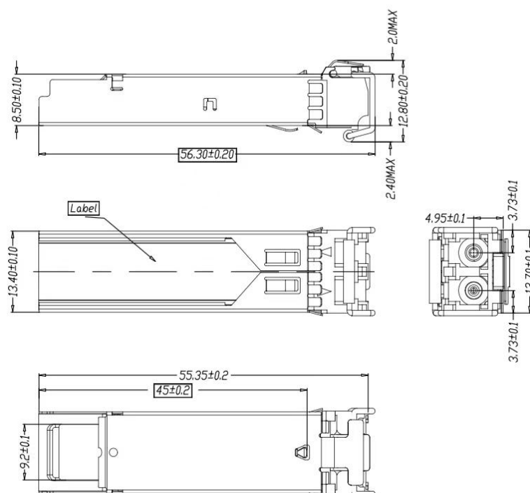
Mechanical Drawing
