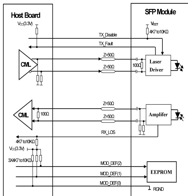
SFP Host Recommended Circuit
