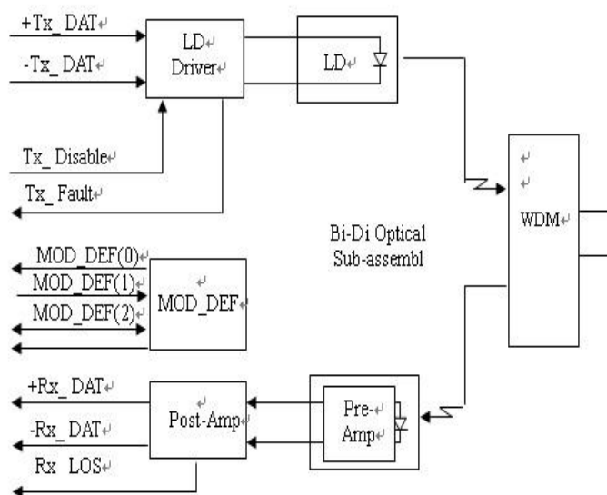
Block Diagram
