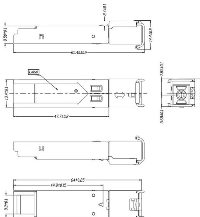
Mechanical Drawing
