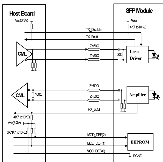
SFP Host Recommended Circuit
