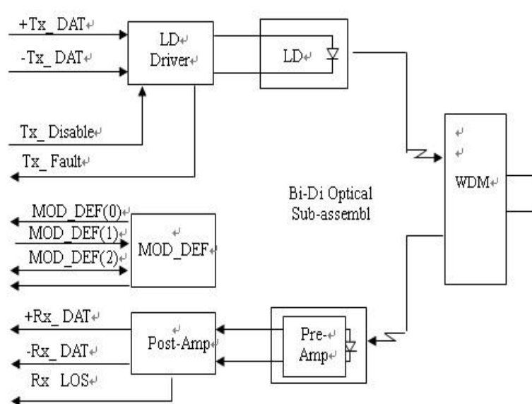
Block Diagram
